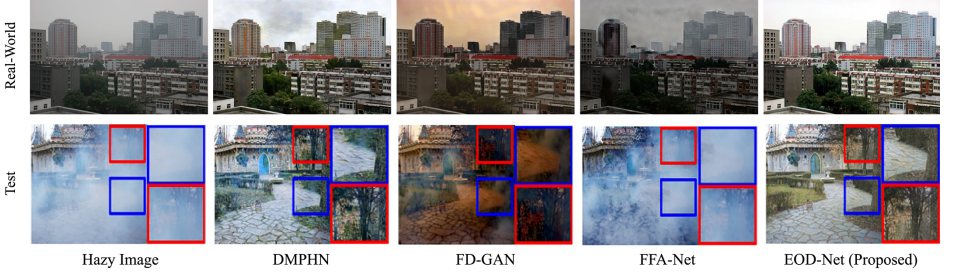
Figure 6: Qualitative comparison on a real-world hazy image (top) and an outdoor test image (bottom).
