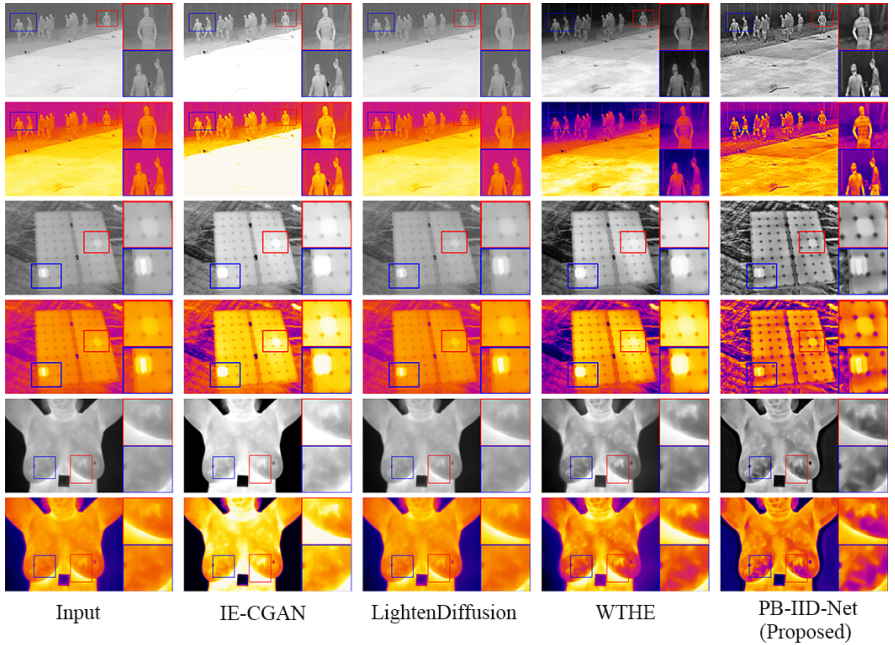
Figure 11: Generalizability of PB-IID-Net: preserving edges, textures, and contrast across diverse domains.
