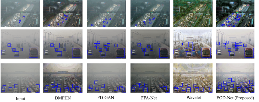
Figure 7: Vehicle detection results compared with SOTA dehazing methods.
